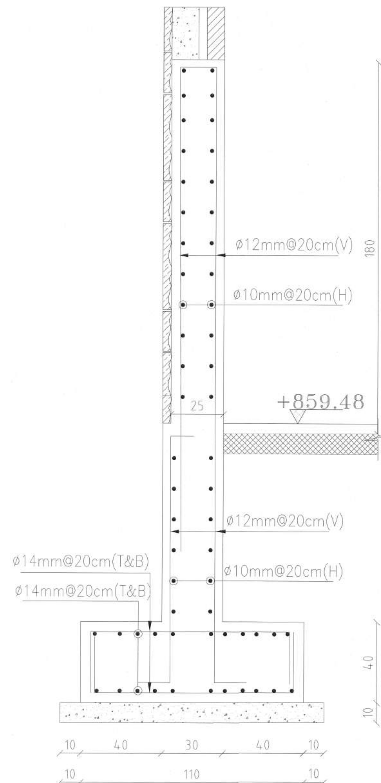
SECTION 3-3 SCALE 1:20
