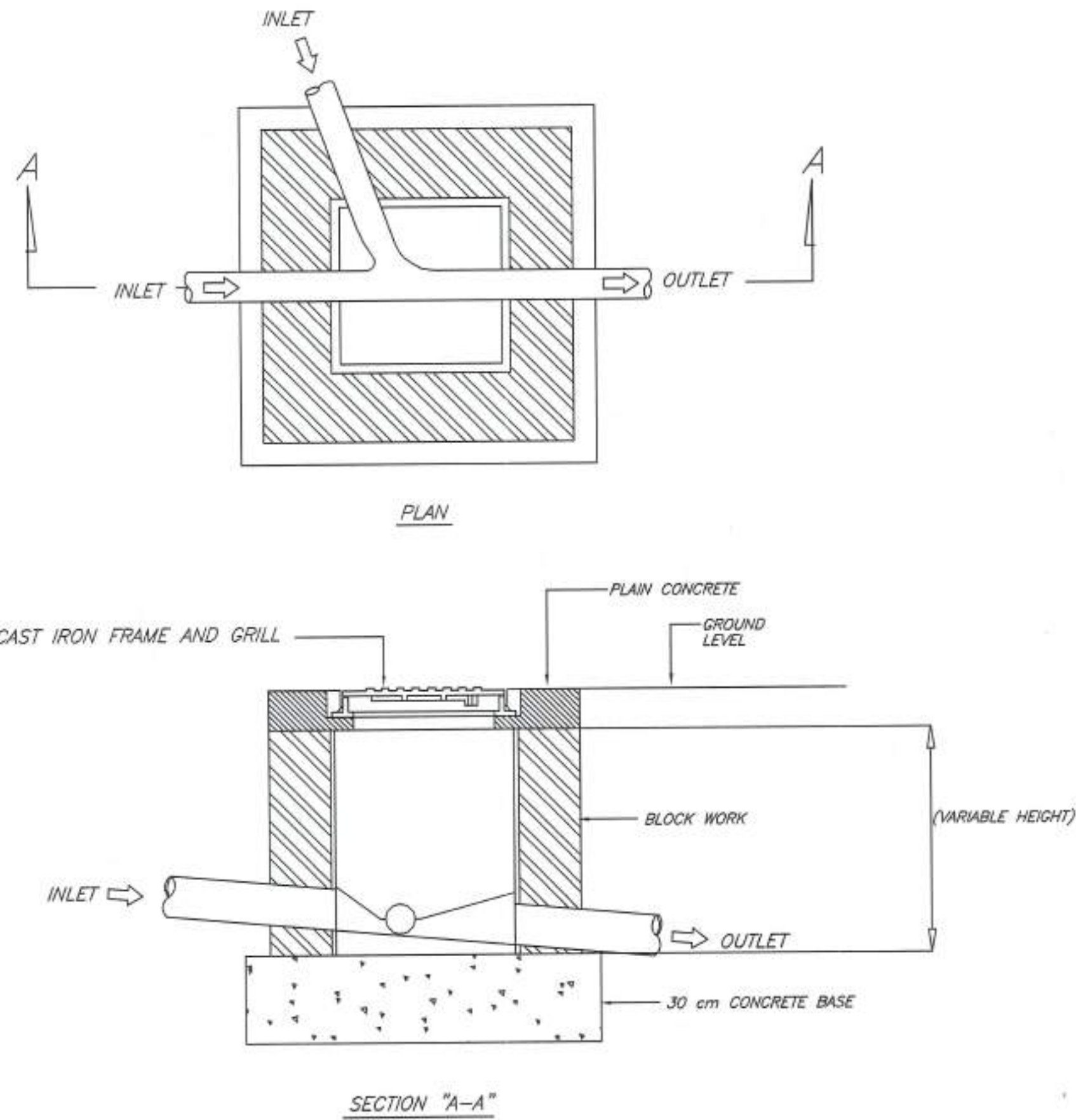
RAIN MANHOLE DETAIL (IC) NOT TO SCALE
