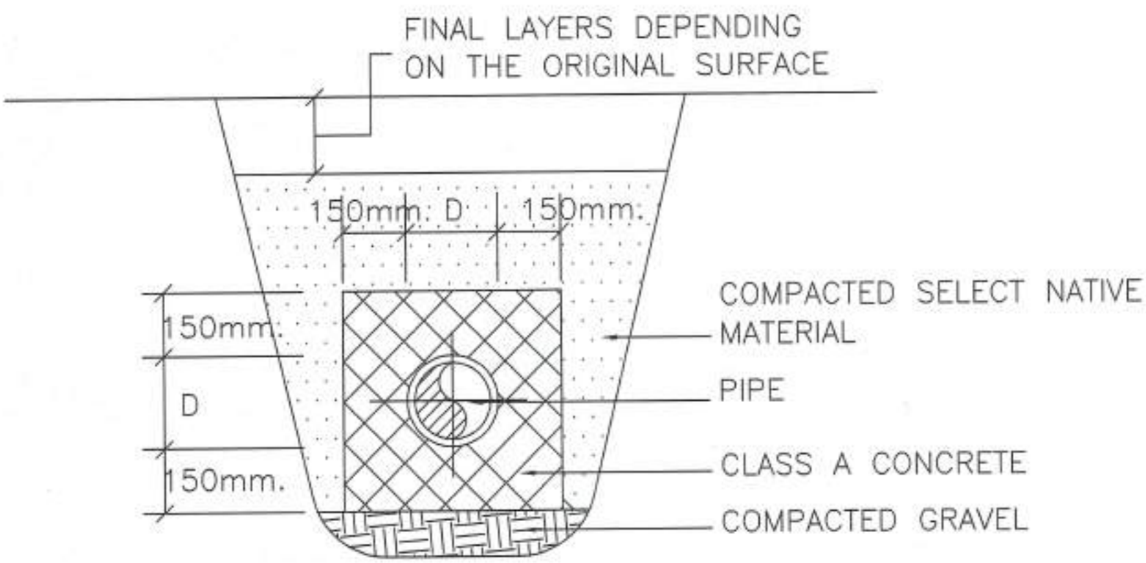
UNDERGROUND DRAINAGE PIPE ENCASEMENT BELOW FOUNDATION & TIE BEAMS
