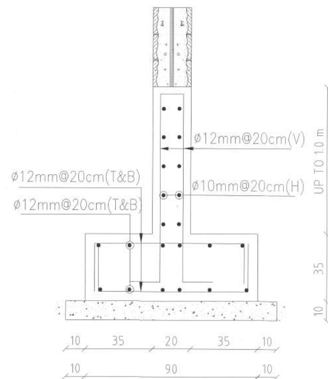
SECTION 2-2 SCALE 1:20
